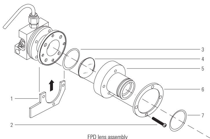
FPD lens assembly
